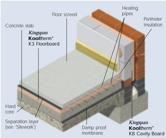
Figure 4 UNDERFLOOR HEATING – INTERMITTENT HEATING CYCLE APPLICATIONS
