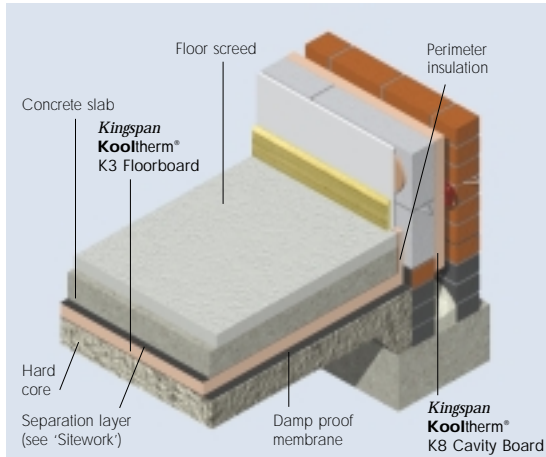
Figure 1 BELOW THE FLOOR SLAB
