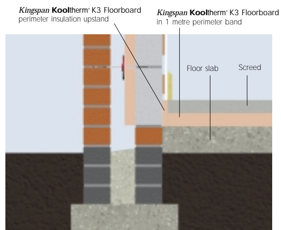
Figure 12 PERIMETER INSULATION
