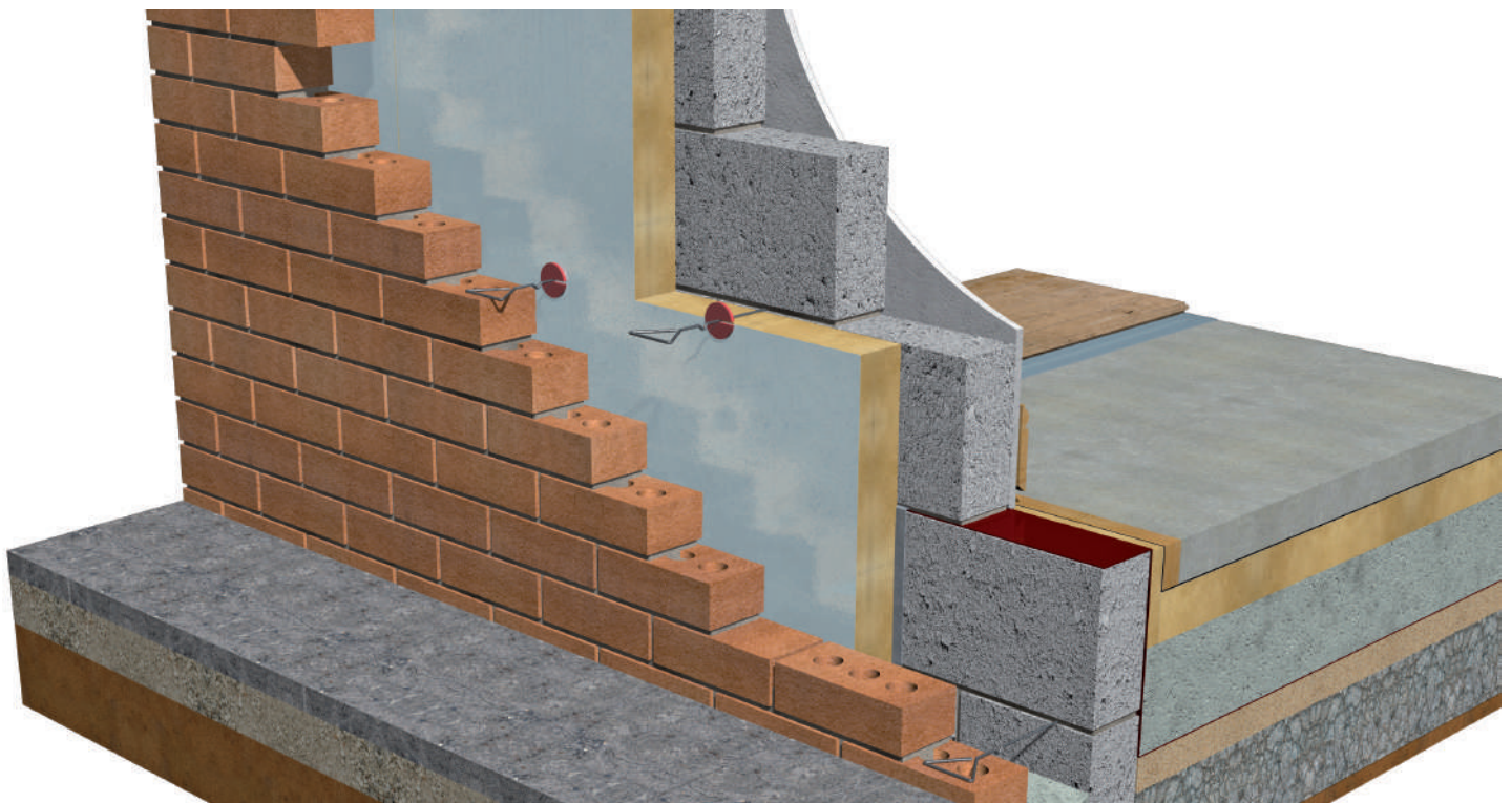
Cavity walls: MC in masonry - partial fill
